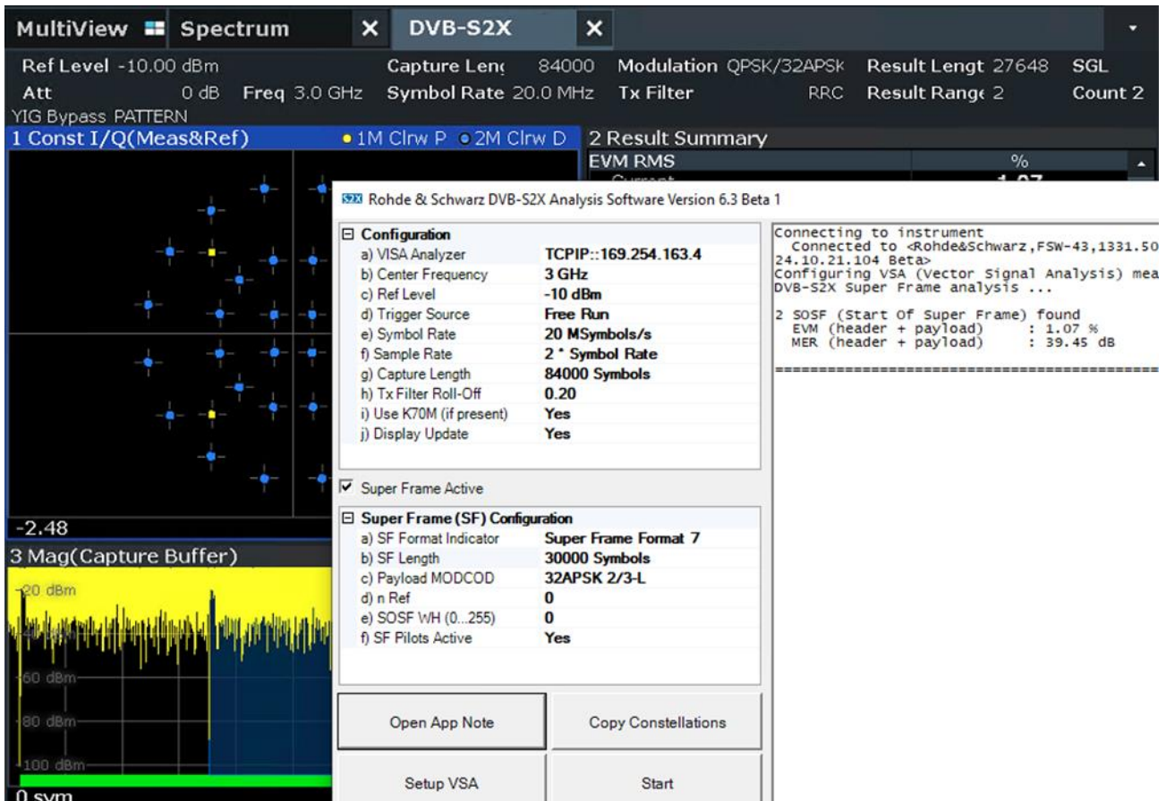
Figure 9 Measurement of an S2X signal with super frame format 7
