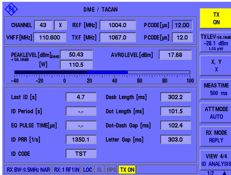
Fig. 9: Identifier analysis
