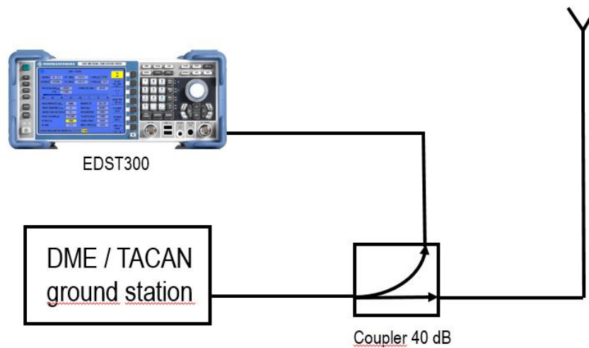
Fig. 6: Test setup for wired measurements on a DME or TACAN station
