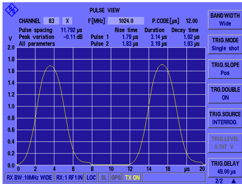
Fig. 8: Time domain measurement of a pulse pair
