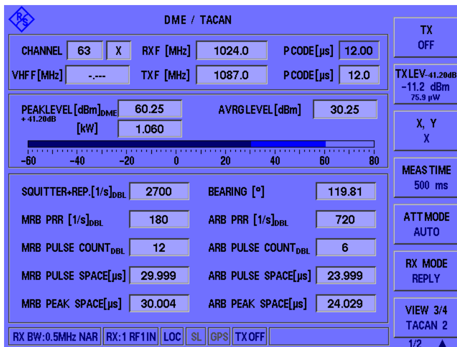
Fig. 10: Analysis of the MRB and ARB
