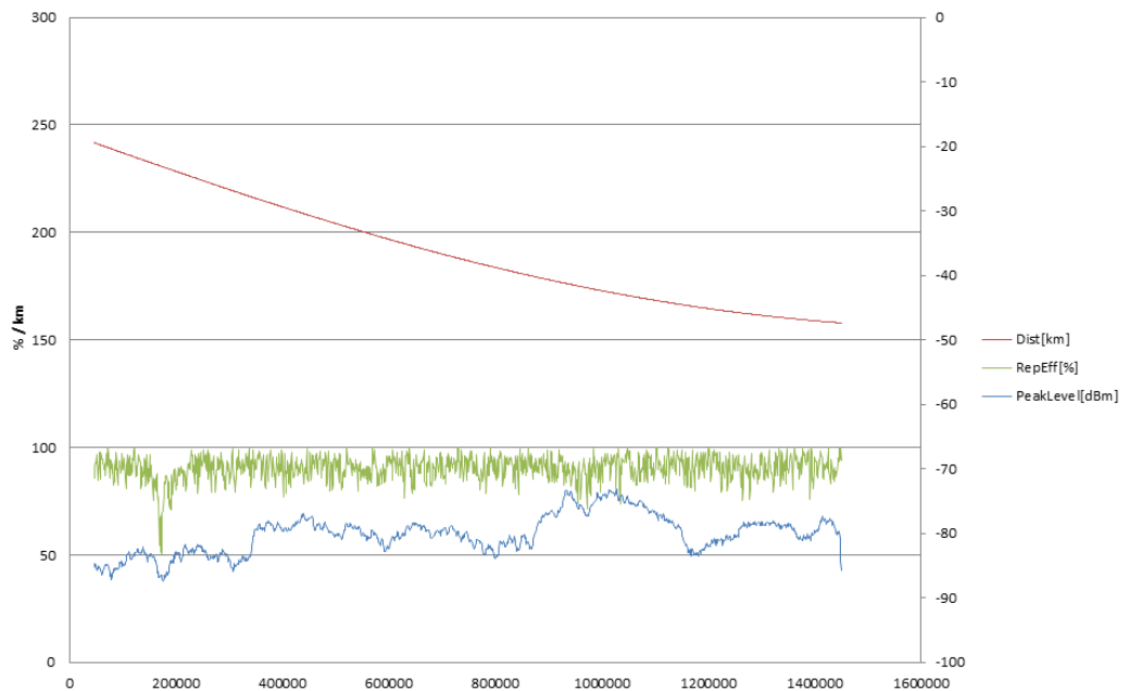
Fig. 20: Results from an MDME flight inspection for one of the DME stations.
