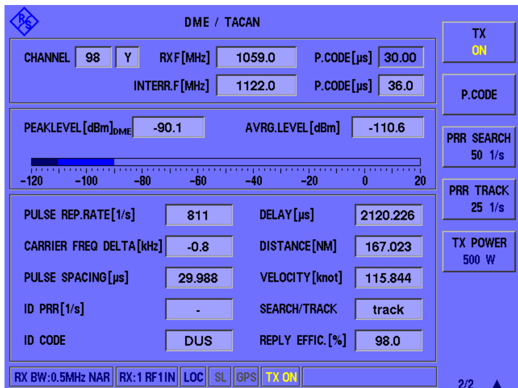
Fig. 13: Measurement results on a DME station (channel 98Y).
