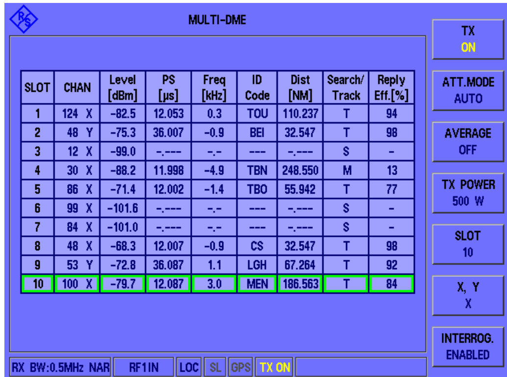
Fig. 17: MDME screen of the R&S® EDS300.
