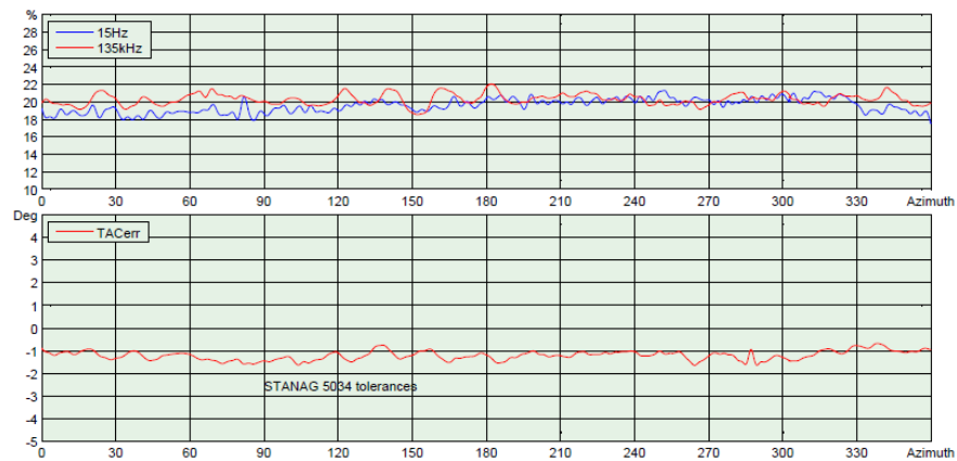
Fig. 21: Results from a TACAN flight inspection.
