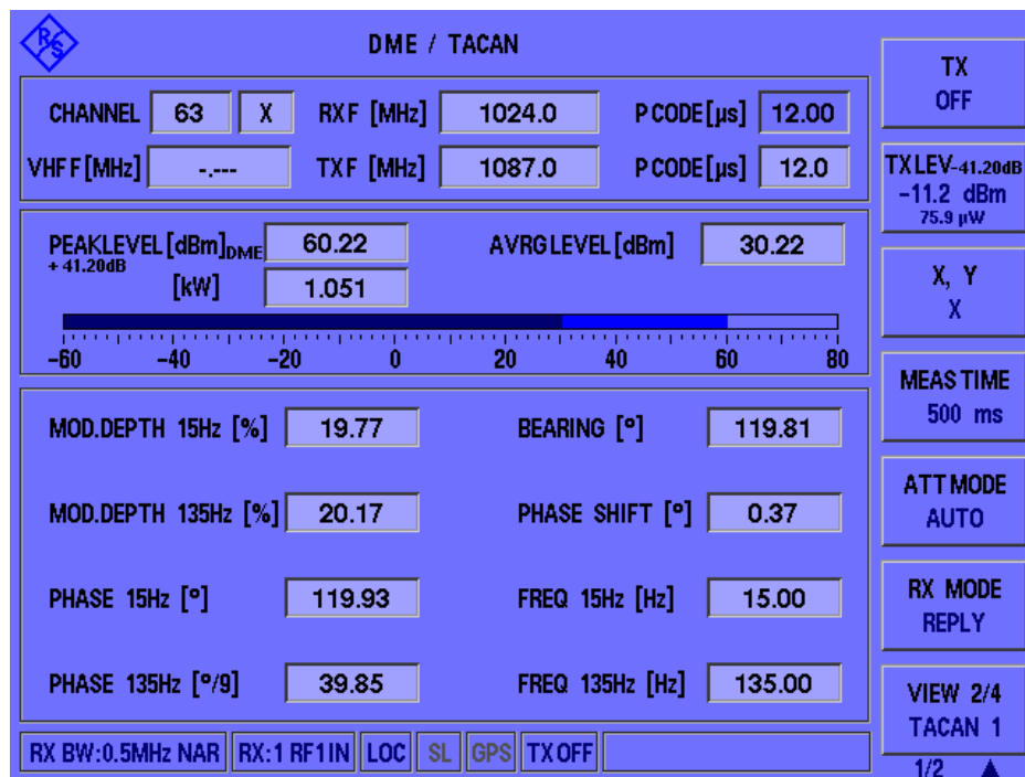
Fig. 19: Modulation depth and bearing measurement
