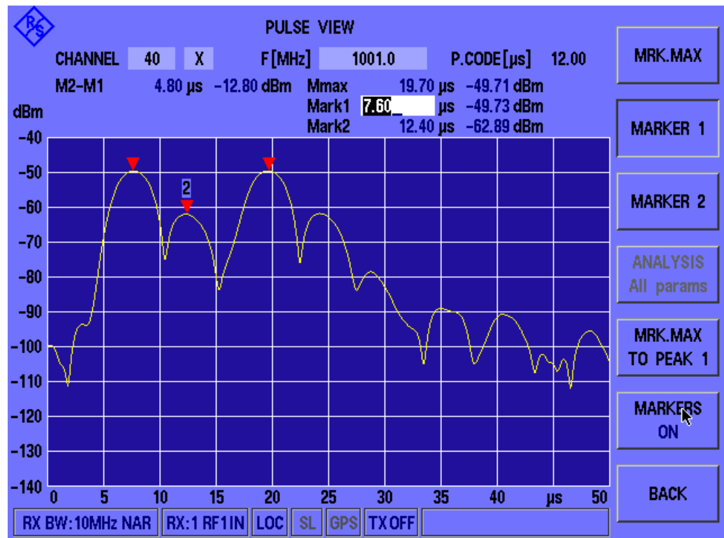
Fig. 15: Analysis of a DME's pulse shape
