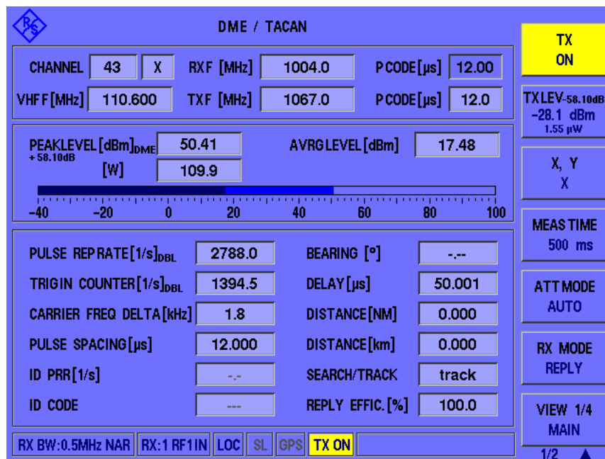
Fig. 7: Result screen of the R&S®EDST300
