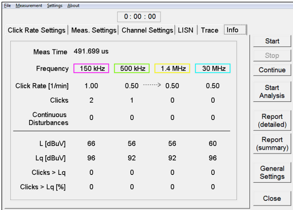
Fig. 14 Information window
