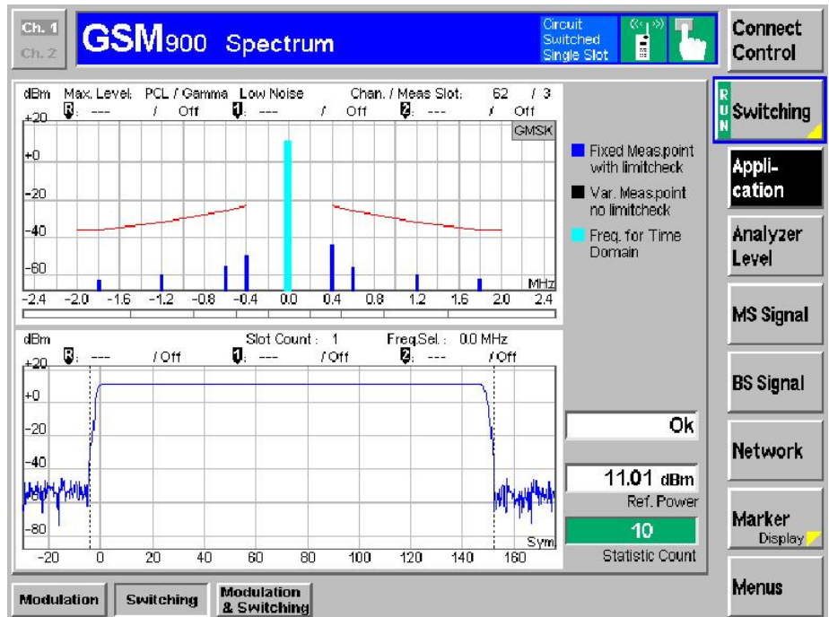
Fig. 15 - Spectrum due to switching
