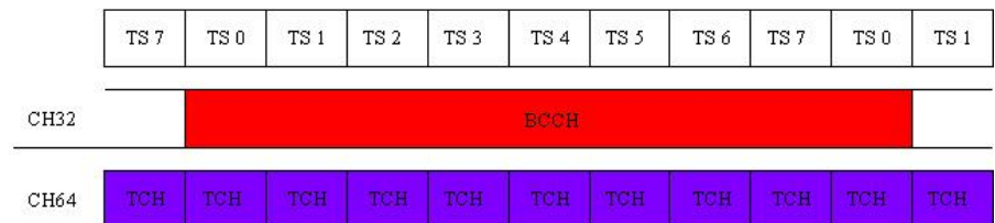
Fig. 4 - Downlink with option B95
