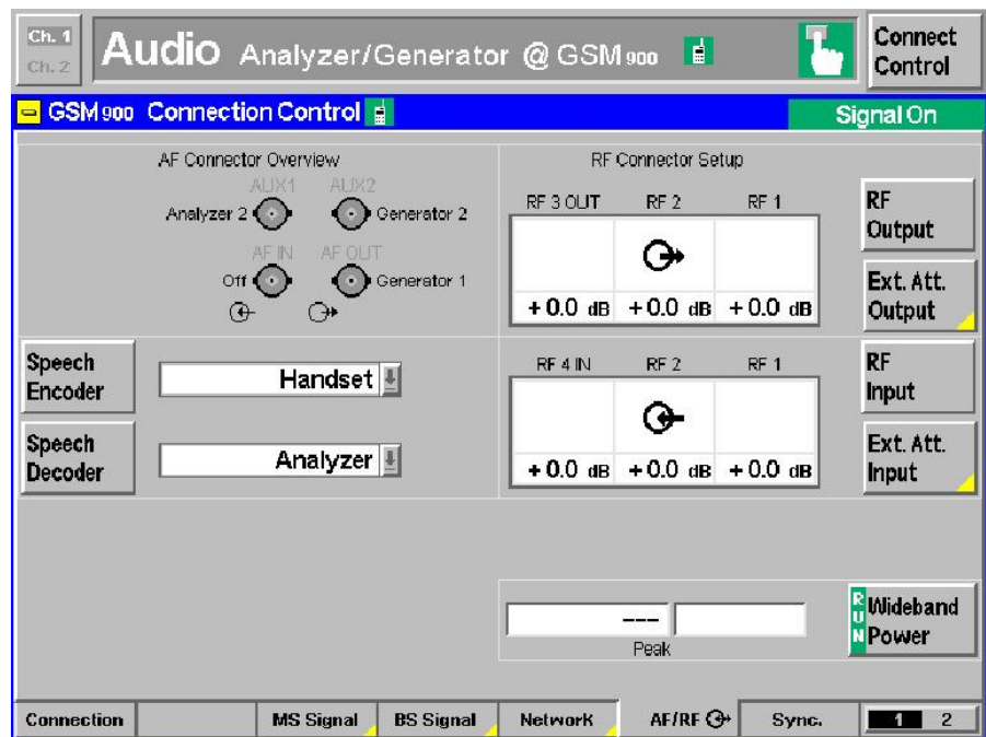
Fig. 20 - Audio uplink setting
