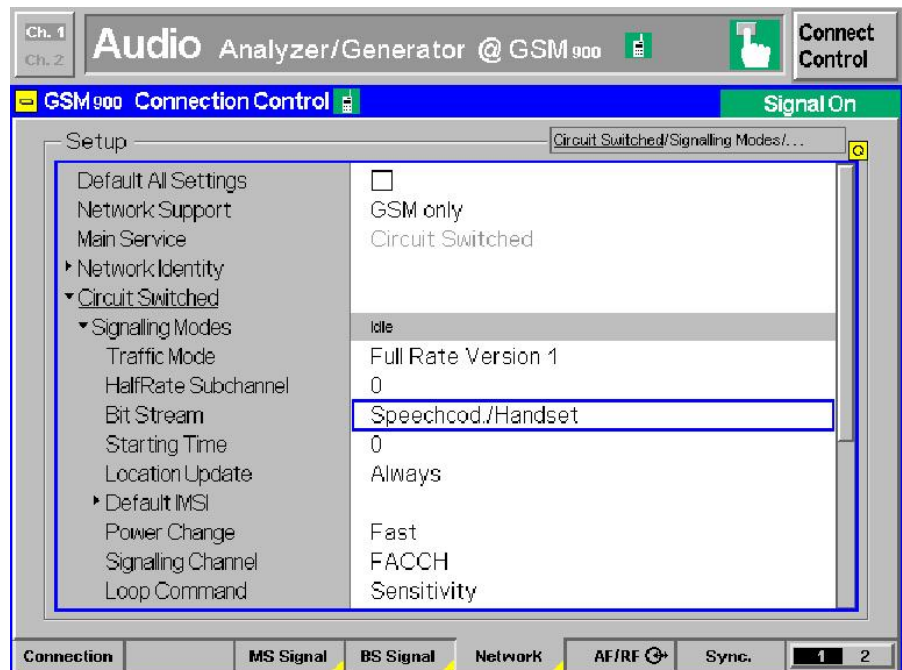
Fig. 18 - Audio setting: Bit Stream
