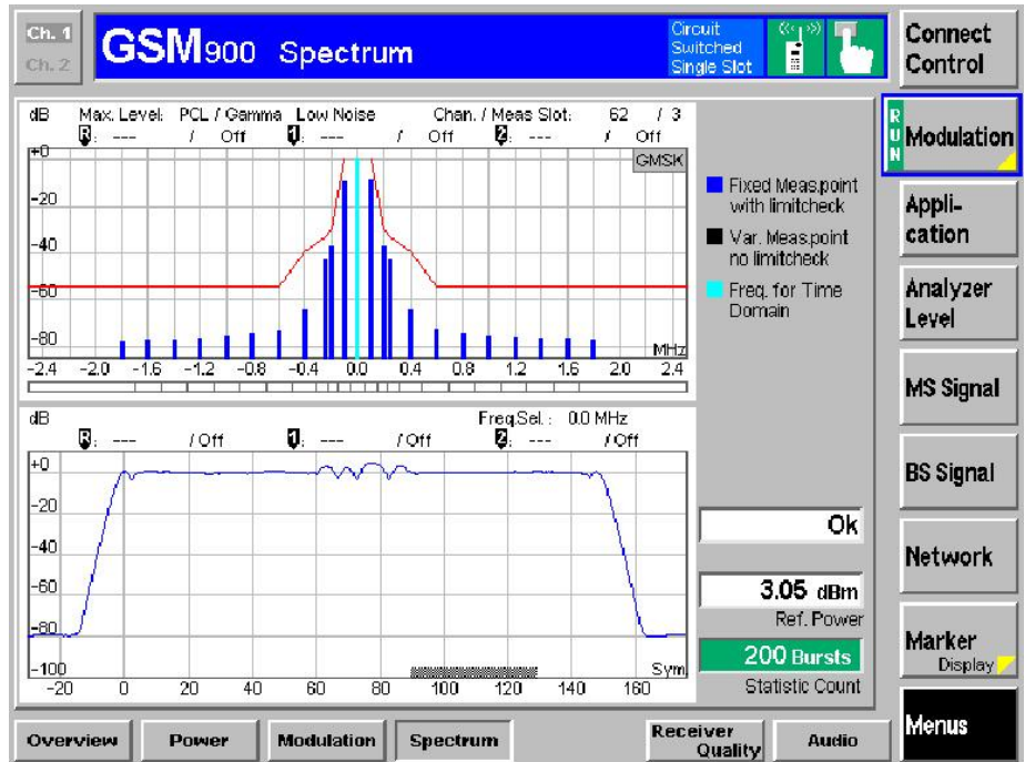
Fig. 14 - Spectrum due to modulation
